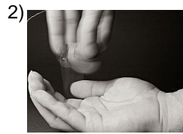
remainder
