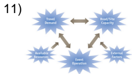
factors
