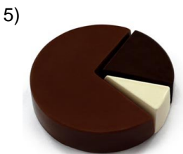
to divide
