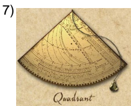
quadrant
