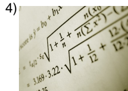
statistics
