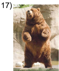
bear
