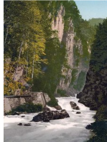
gully, ravine
